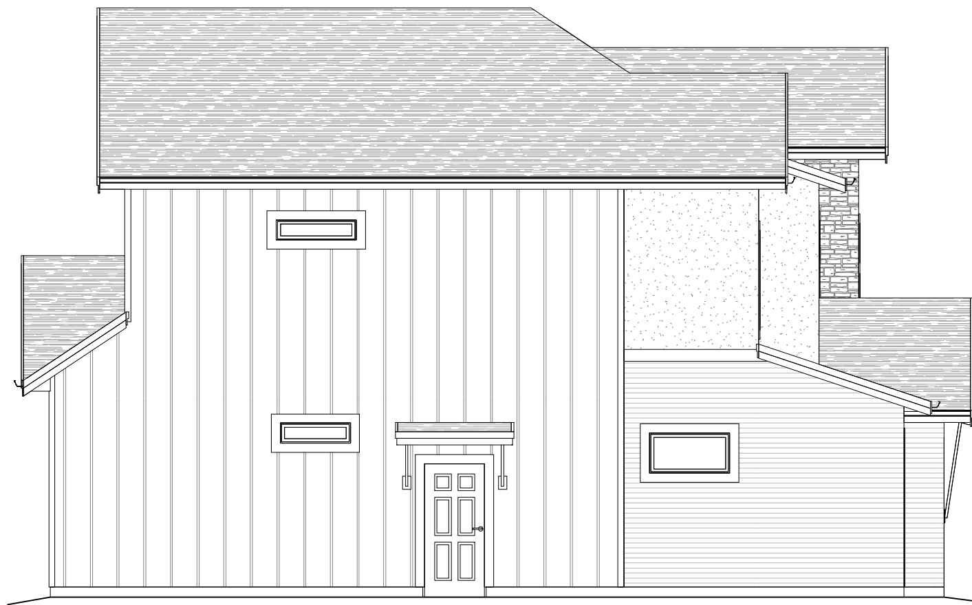
③ CONCEPT LEFT ELEVATION 1/4" = 1'-0"
