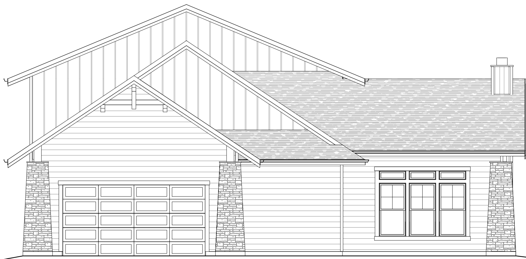
③ CONCEPT LEFT ELEVATION 1/4" = 1'-0"
