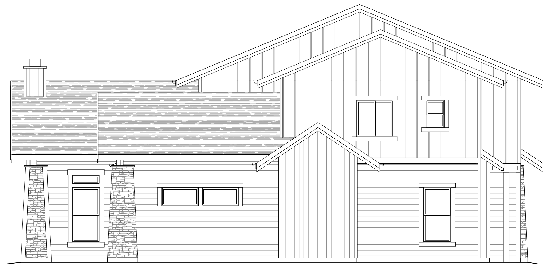
④ CONCEPT RIGHT ELEVATION 1/4" = 1'-0"
